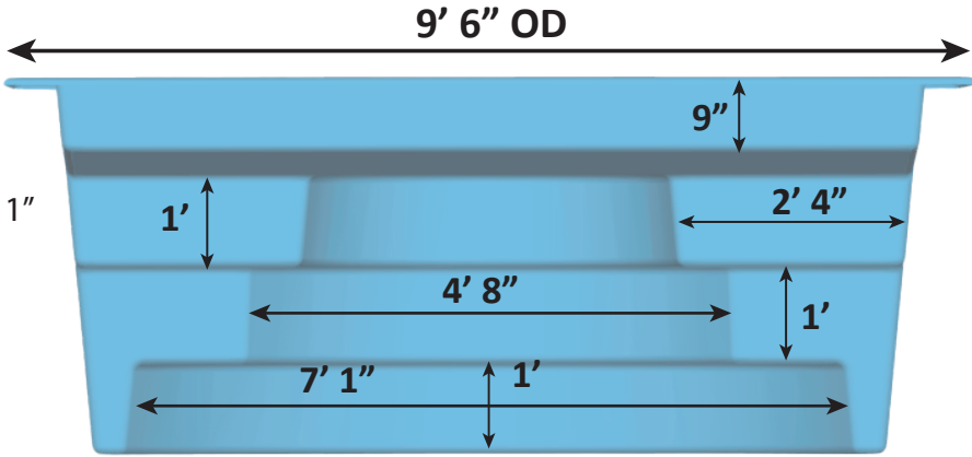
Step End View
